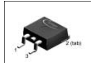
PG-TO263-3-2
