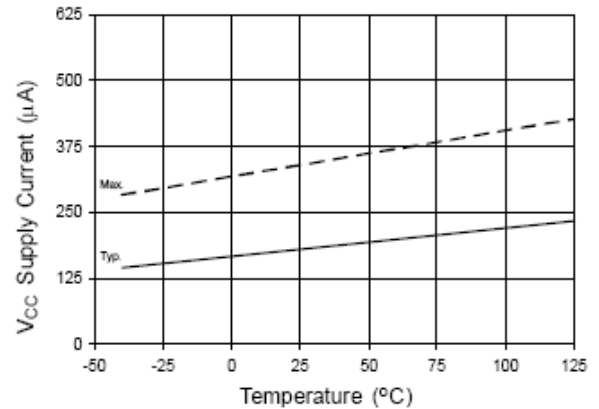
Figure 18A. V CC Supply Current vs. Temperature
