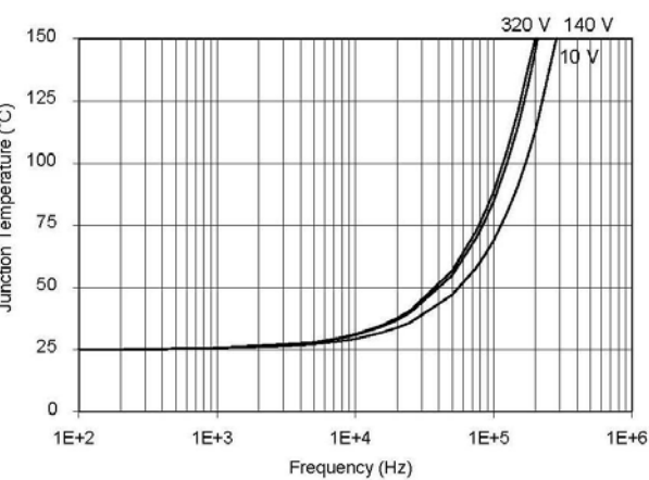
Figure 43. IRS2117/IRS2118 T_J vs. Frequency (IRFPE50) R_{GATE}=10\Omega , V_{CC}=15V
