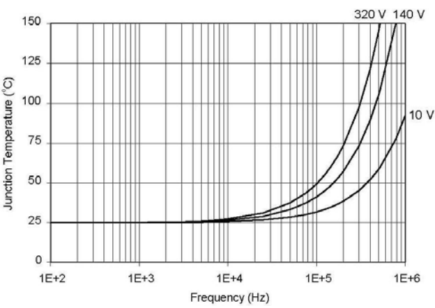
Figure 41. IRS2117/IRS2118 T_J vs. Frequency (IRFBC30) R_{GATE}=22\Omega , V_{CC}=15V
