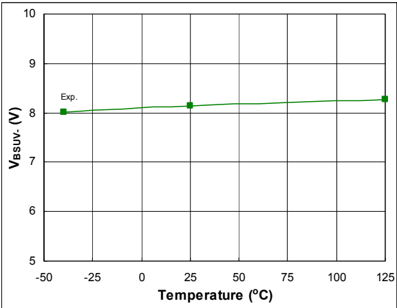
Figure 57: V BSUV- vs. temperature
