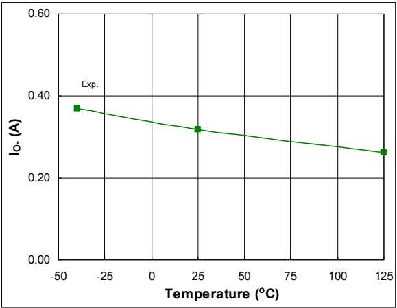
Figure 53: I O- vs. temperature
