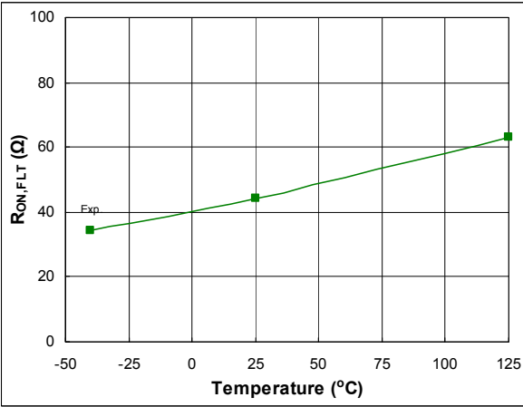
Figure 61: R ON,FLT vs. temperature
