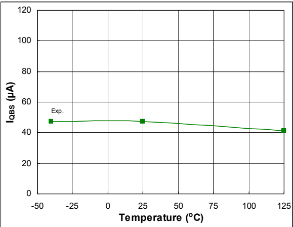
Figure 51: I QBS vs. temperature
