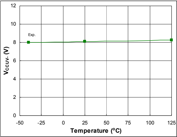
Figure 55: V CCUV- vs. temperature
