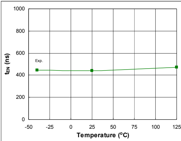
Figure 45: t EN vs. temperature
