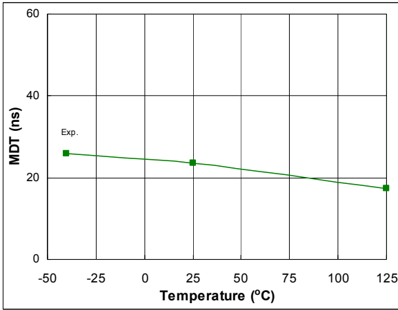
Figure 47: MDT vs. temperature
