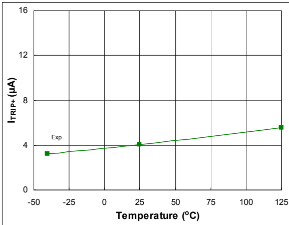
Figure 49: I TRIP+ vs. temperature
