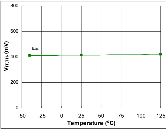
Figure 59: V IT,TH- vs. temperature
