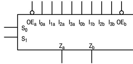
Figure 2. Logic Symbol
