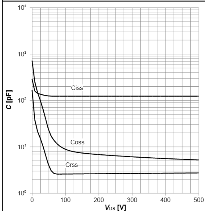
Diagram 13: Typ. capacitances
