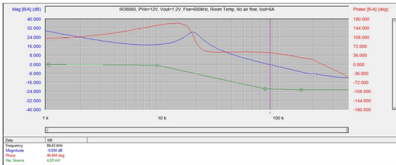
Figure 52: Bode Plot at 6A load Bandwidth = 84.4kHz, Phase Margin = 46.6°
