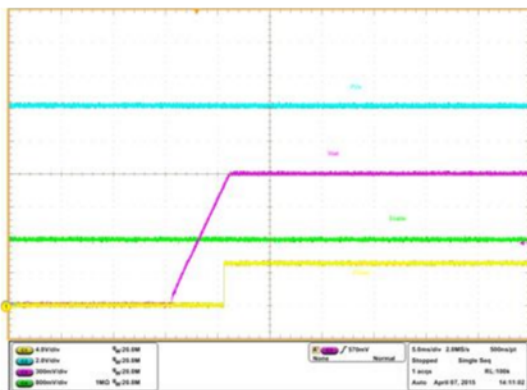
Figure 43: Operation 80, Turn ON without margining, 6A load
