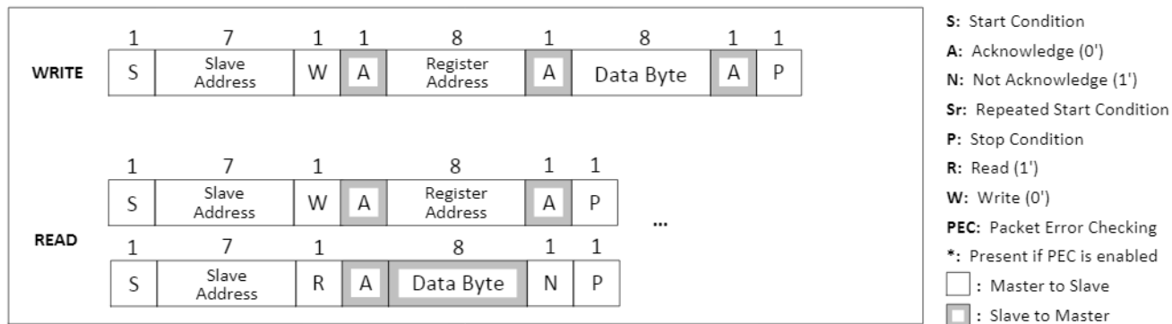
Figure 57: I2C Format
