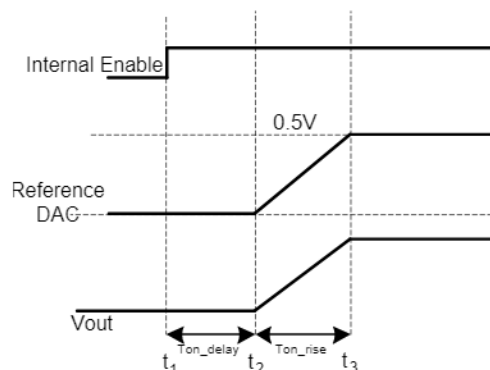
Figure 18: DAC2 (VREF) Soft start
