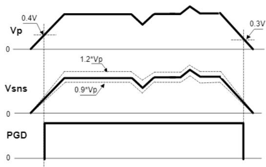
Figure 30: Vp Tracking ( \overline{\text{Track\_En}} = 0\text{V} )
