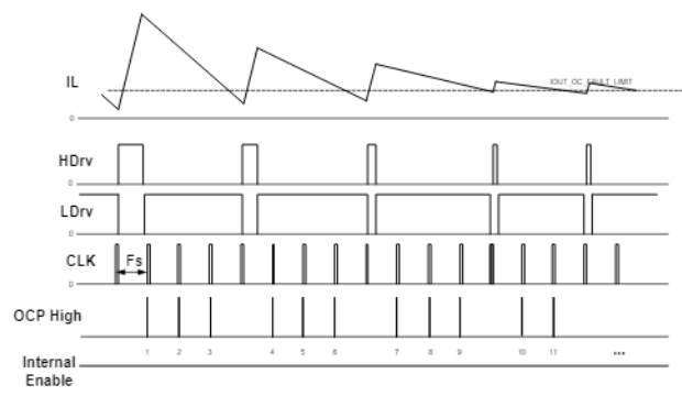
Figure 23: Constant current limiting.
