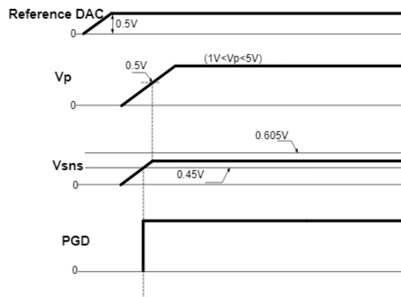
Figure 31: Vp Sequencing (100 kOhm from \overline{\text{Track\_En}} to P1V8)
