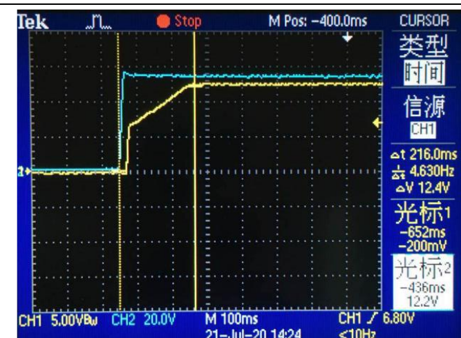
Output response & load (12V / 2A)
