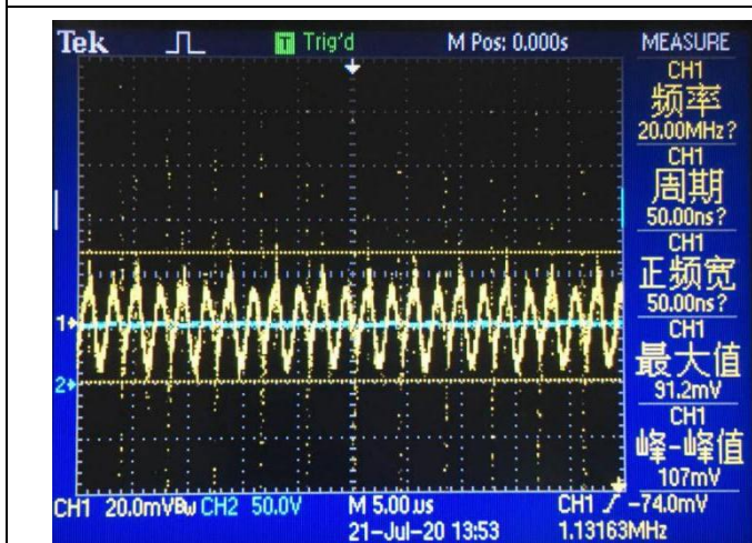
Noise ( V_{IN} = 57V , I_O = 2.5A , 5 ~ 20MHz bandwidth)
