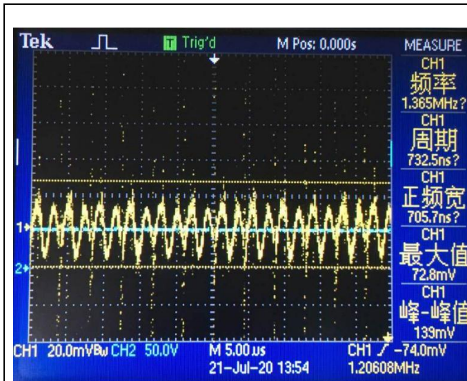
Noise ( V_{IN} = 37V , I_O = 2.5A , 5 ~ 20MHz bandwidth)
