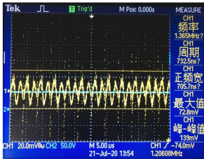
Noise ( V_{IN} = 37V , I_O = 2.5A , 5 ~ 20MHz bandwidth)
