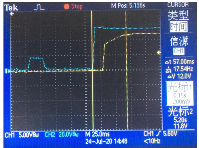
Output response & load (12V / 0.5A)
