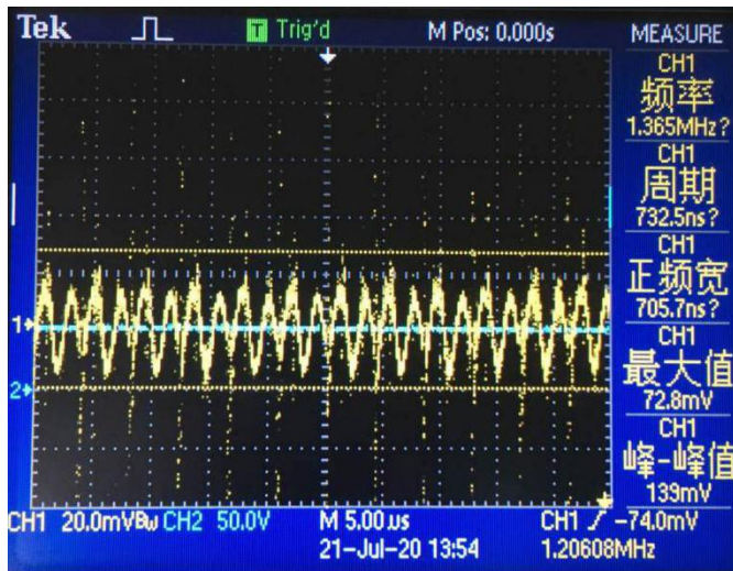
Noise ( V_{IN} = 42V , I_O = 3.75A , 5 ~ 20MHz bandwidth)
