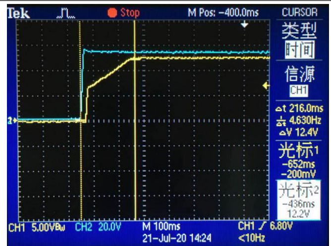
Output response & load (12V / 3.75A)
