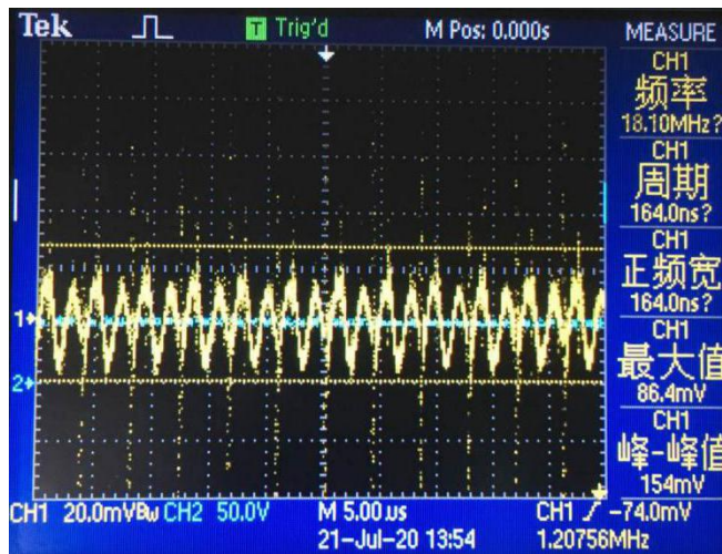
Noise ( V_{IN} = 48V , I_O = 3.75A , 5 ~ 20MHz bandwidth)
