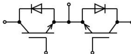
Internal Circuit
