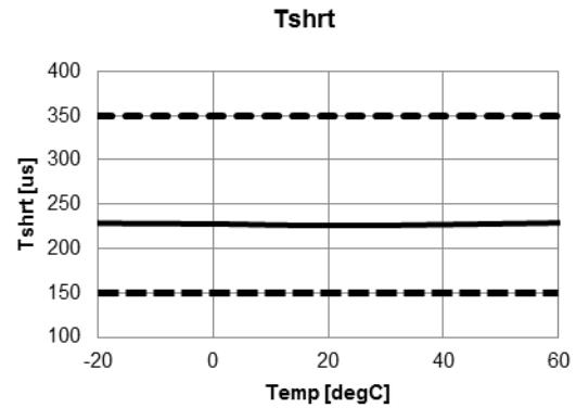
Figure 19. T SHRT vs. Temperature
