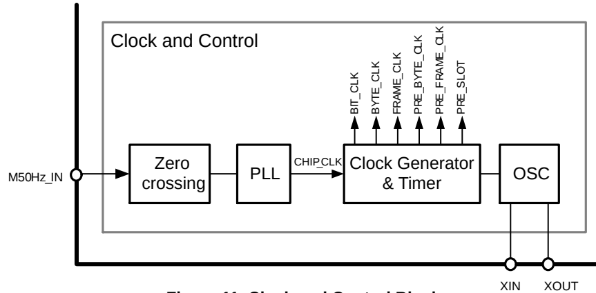
Figure 11. Clock and Control Block
