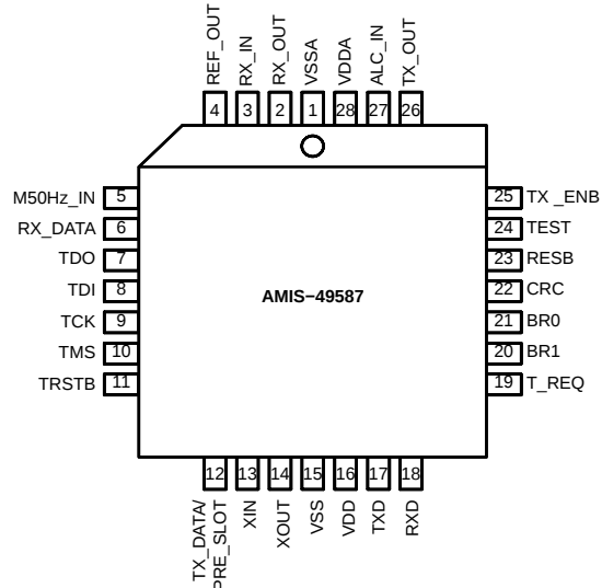
Figure 2. Pinout
