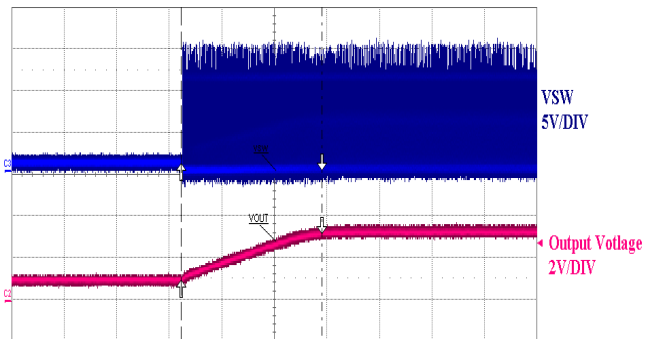
Figure 8. 3.3 V Turn on into 1 V Pre-Bias 1 \text{ms}/\text{DIV}
