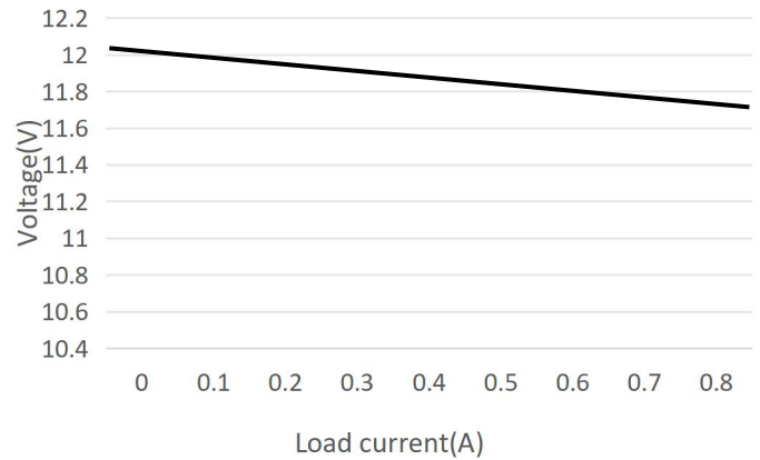
Output voltage (input 48V)
