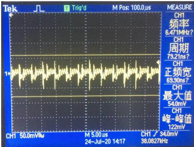
Noise ( V_{IN} = 42V , I_O = 0.5A , 5 ~ 20MHz bandwidth)
