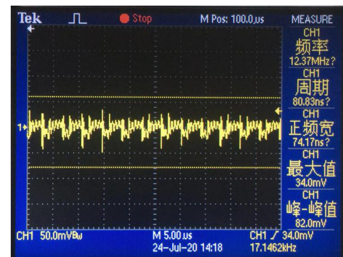
Noise ( V_{IN} = 57V , I_O = 0.5A , 5 ~ 20MHz bandwidth)
