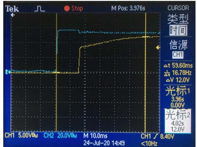
Output response & load (12V / 0.5A)
