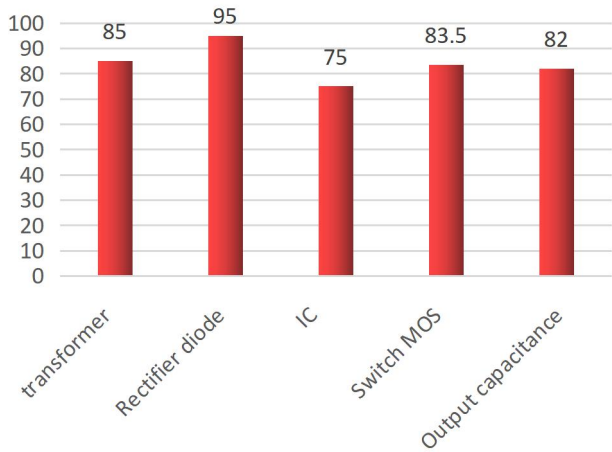
Efficiency (Vout = 12 V)
