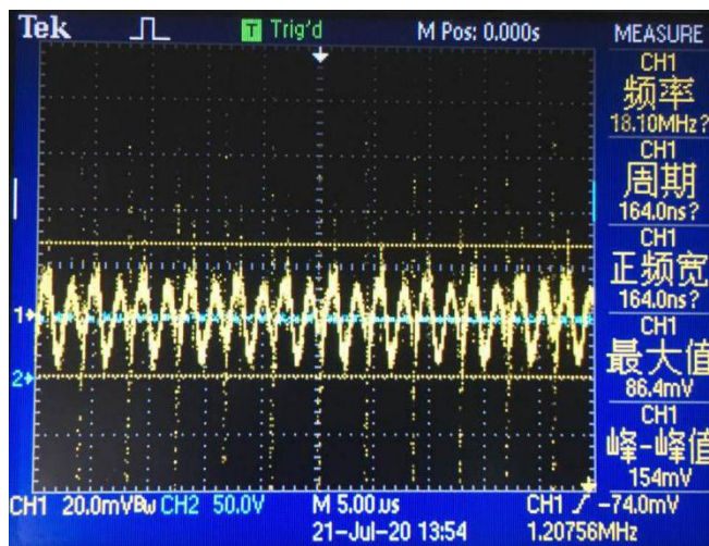
Noise ( V_{IN} = 48V , I_O = 1.25A , 5 ~ 20MHz bandwidth)
