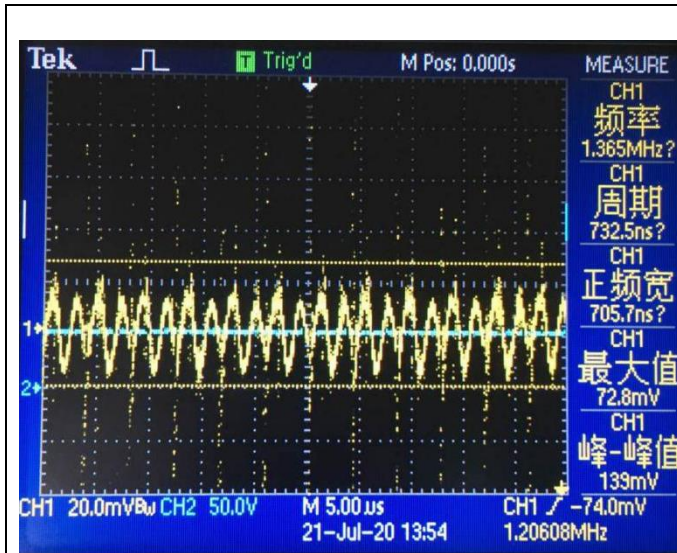
Noise ( V_{IN} = 42V , I_O = 5A , 5 ~ 20MHz bandwidth)
