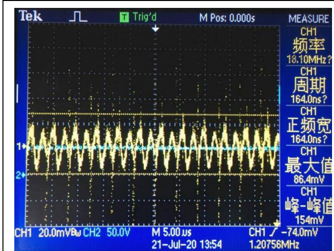
Noise ( V_{IN} = 48V , I_O = 5A , 5 ~ 20MHz bandwidth)
