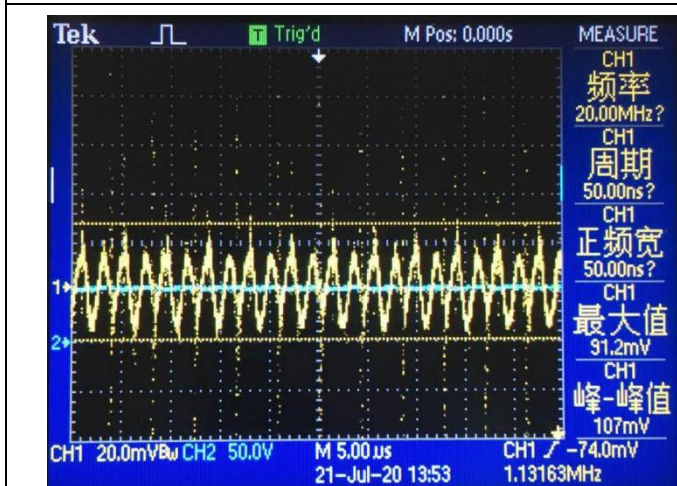
Noise ( V_{IN} = 57V , I_O = 5A , 5 ~ 20MHz bandwidth)
