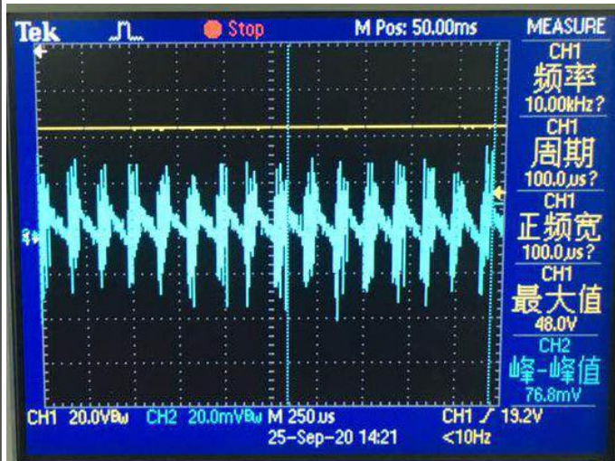
Noise ( V_{IN} = 48V , I_O = 0.01A , 5 ~ 20MHz bandwidth)
