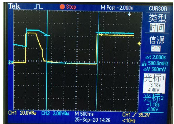
Output response & load (5V / 0.6A)
