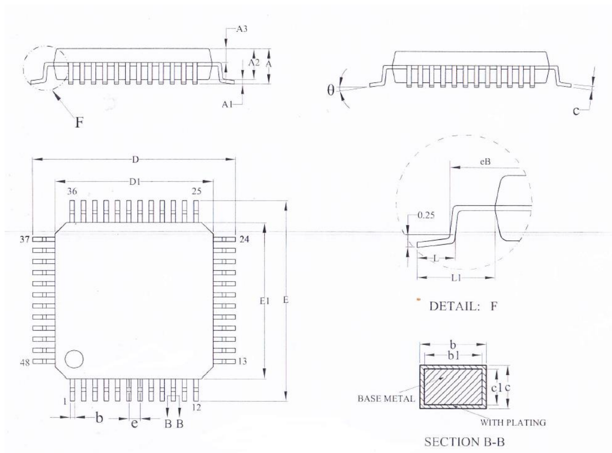
Figure 5-1. LQFP48 package outline
