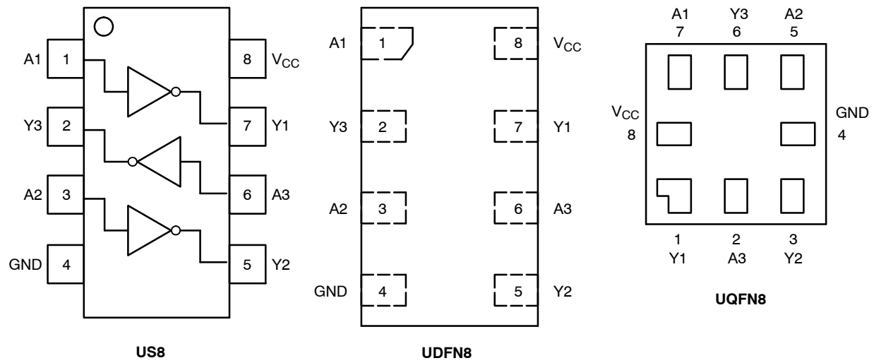
Figure 2. Pinout
