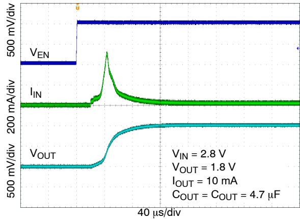
Figure 27. Enable Turn-on Response – V_{OUT} = 1.8\text{ V} , C_{OUT} = 4.7\ \mu\text{F}
