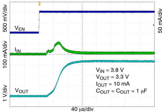
Figure 28. Enable Turn-on Response – V_{OUT} = 3.3\text{ V} , C_{OUT} = 1\ \mu\text{F}
