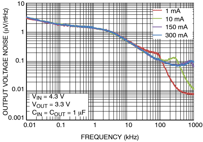
Figure 25. Output Voltage Noise Spectral Density for V_{OUT} = 3.3\text{ V} , C_{OUT} = 1\ \mu\text{F}
