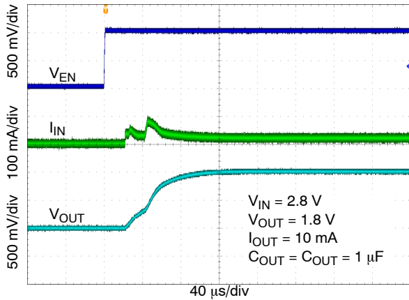
Figure 26. Enable Turn-on Response – V_{OUT} = 1.8\text{ V} , C_{OUT} = 1\ \mu\text{F}
