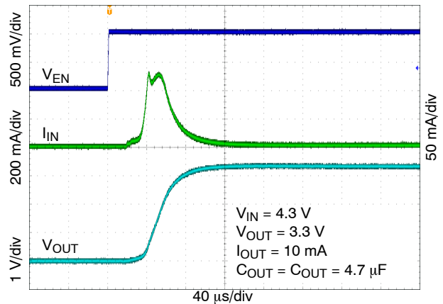
Figure 29. Enable Turn-on Response – V_{OUT} = 3.3\text{ V} , C_{OUT} = 4.7\ \mu\text{F}
