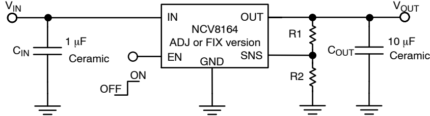
Figure 16. Adjustable Variant Application
