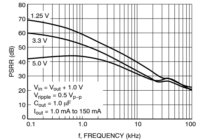
Figure 30. Power Supply Ripple Rejection vs. Frequency
