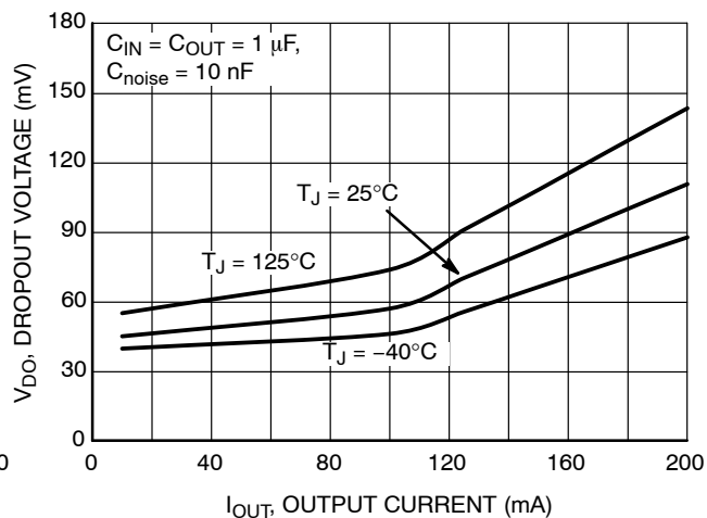
Figure 9. Dropout Voltage vs. Output Current, V_{OUT} = 3.3\text{ V}
