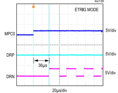
HAPTIC DRIVER TIME FROM MPC0 ASSERTION TO EXTRIG VIBRATION
