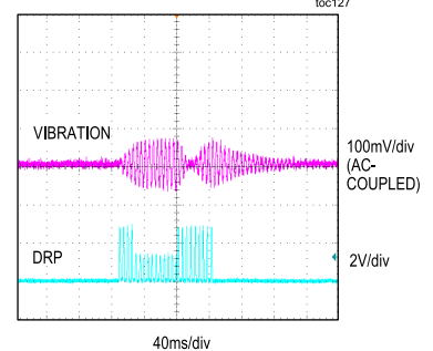
HAPTIC DRIVER LRA CLICK AND BOUNCE
