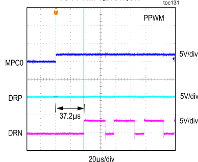
HAPTIC DRIVER TIME FROM MPC0 ASSERTION TO PPWM VIBRATION
