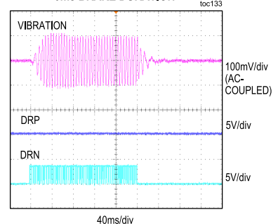
HAPTIC DRIVER 200ms ERM DRIVE 0ms BRAKE DURATION
