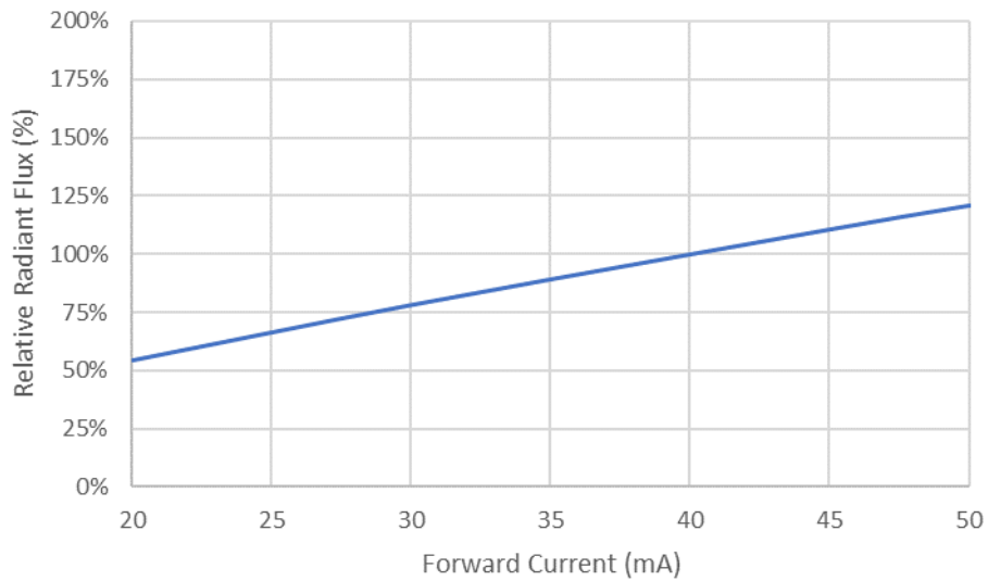
Fig 3. Forward Current vs. Relative Radiant Flux
