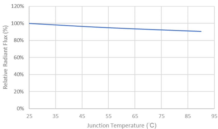
Fig 5. Junction Temperature vs. Relative Radiant Flux
