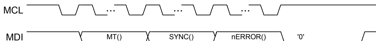
Figure 15: SSI Multitrurn Interface Operation
