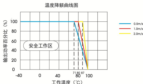
VCB4812EBO-100WR3 (Vin=48V)
