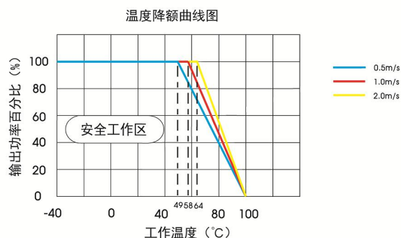
VCB4824EBO-100WR3 (Vin=48V)
