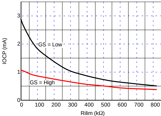
Figure 13. Over Current Threshold versus R_{LIM} 2.85 A Version
