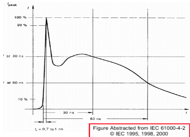
Figure 16. IEC 61000-4-2 Electrostatic Discharge
