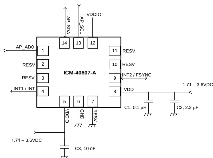
Figure 7. ICM-40607-A Application Schematic (I 2 C Interface to Host)
