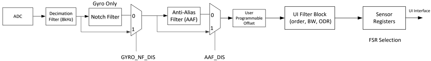
Figure 10. ICM-40607-A Signal Path
