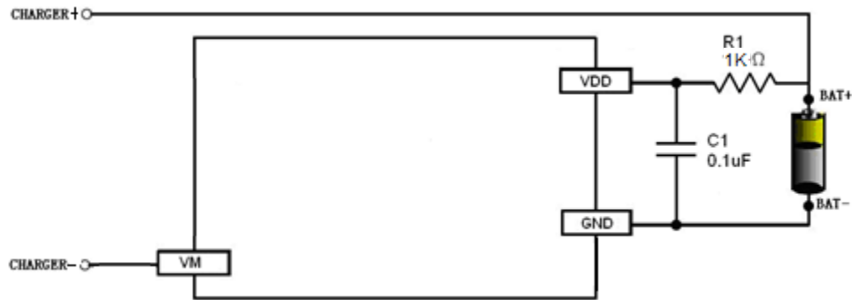
Fig 6 XB7608GJ in a Typical Battery Protection Circuit
