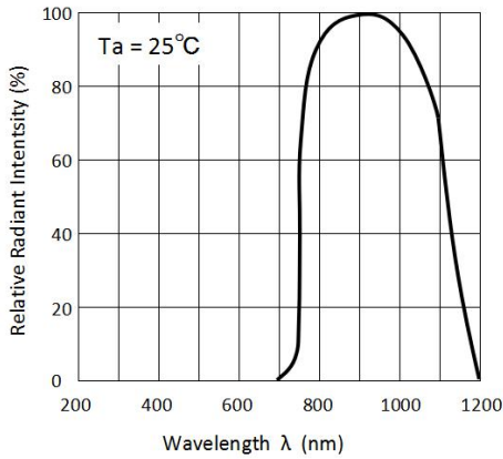
Fig.1 Spectral Distribution
