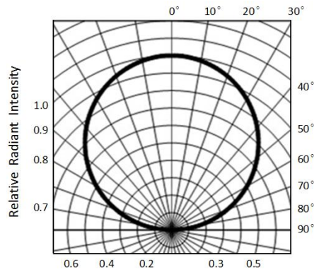
Fig.6 RADIATION CHARACTERISTICS
