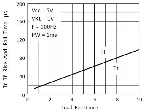
Fig.5 RISE AND FALL TIME VS. LOAD RESISTANCE
