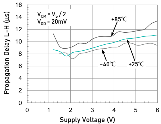
Propagation Delay L-H ( t_{PD,L-H} ) vs. Supply Voltage
