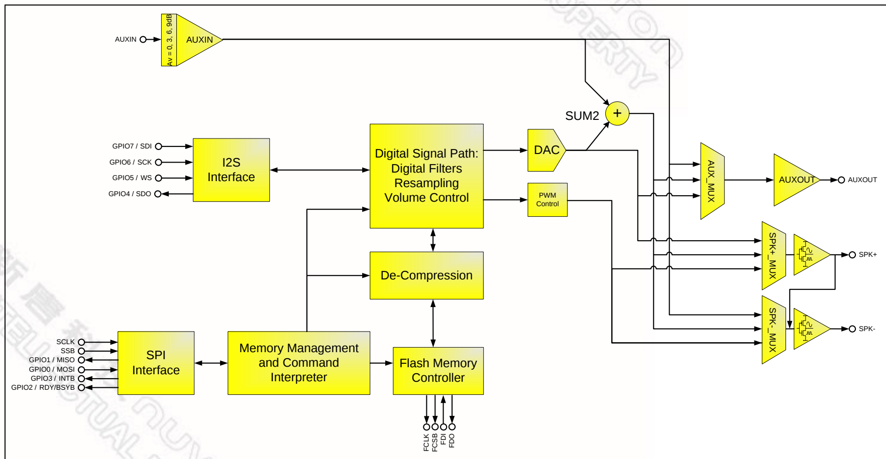
Figure 3-1 ISD3800 Block Diagram
