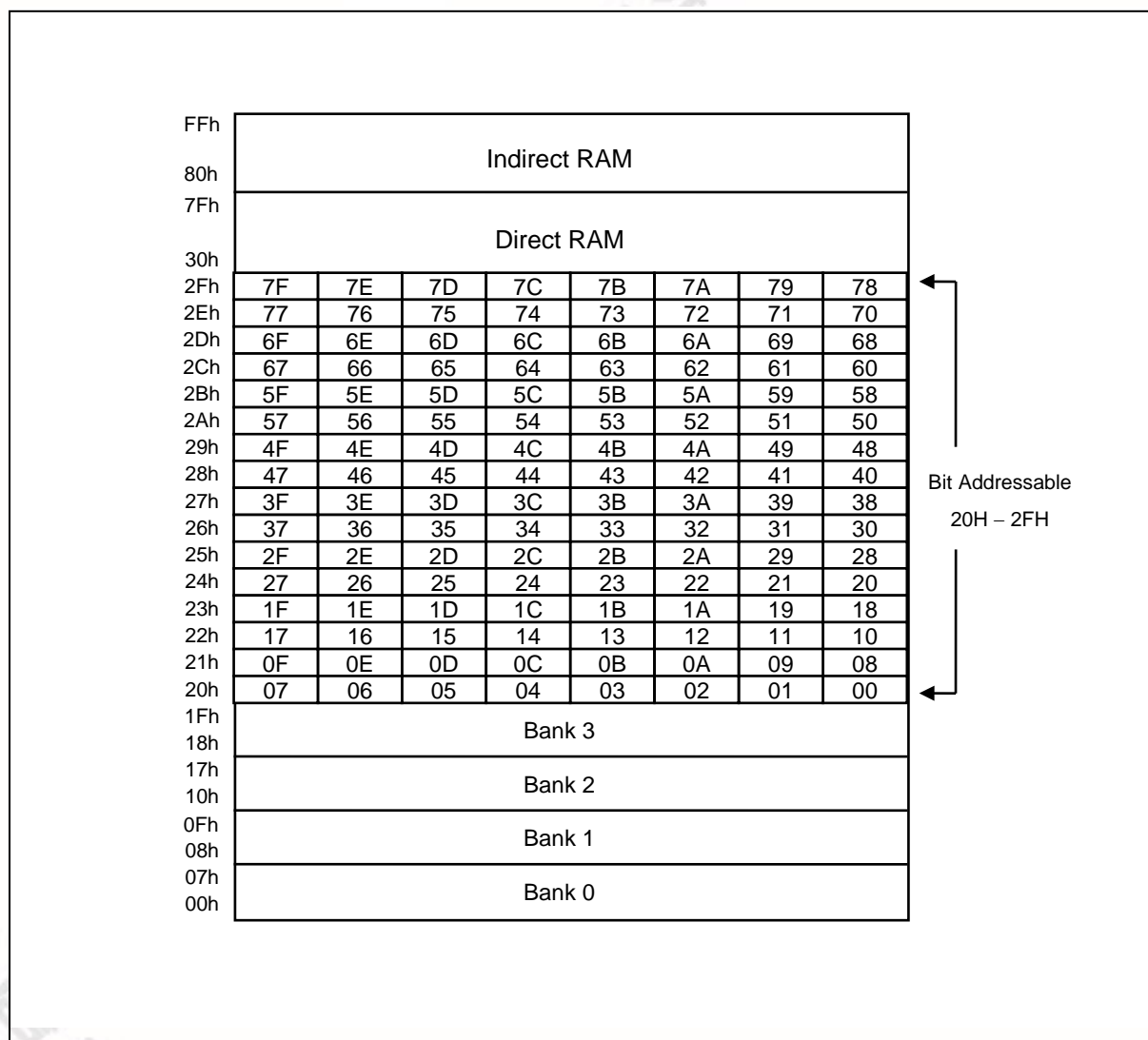
Figure 2. Scratchpad RAM / Register Addressing
