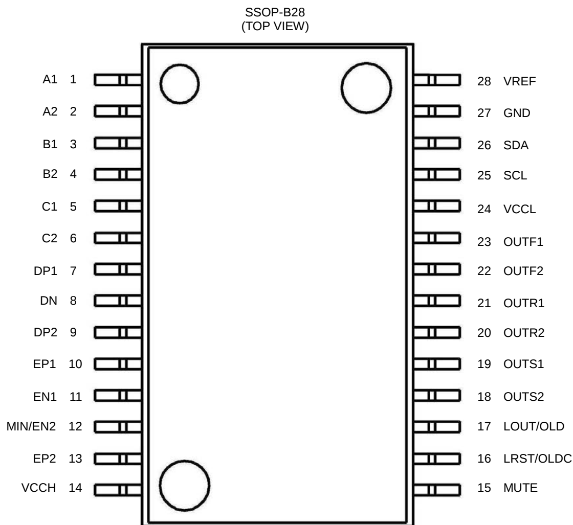
Figure 2. Pin configuration
