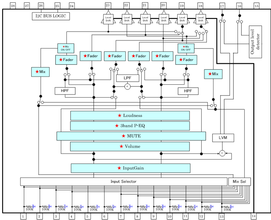
Figure 3. Block Diagram
