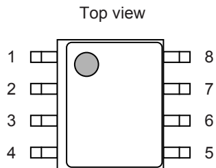
Figure 2 S-35391A-J8T1x
