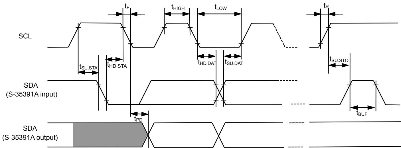
Figure 8 Bus Timing
