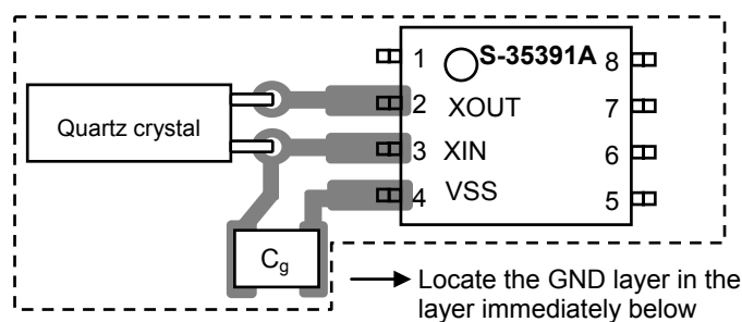
Figure 49 Connection Diagram 1
