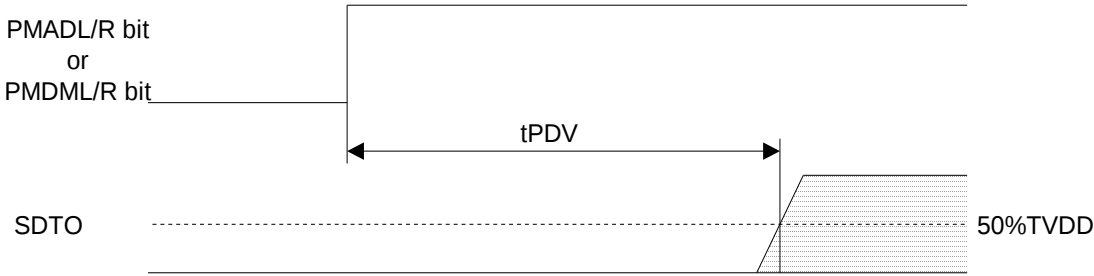
Figure 13. Power Down & Reset Timing 2
