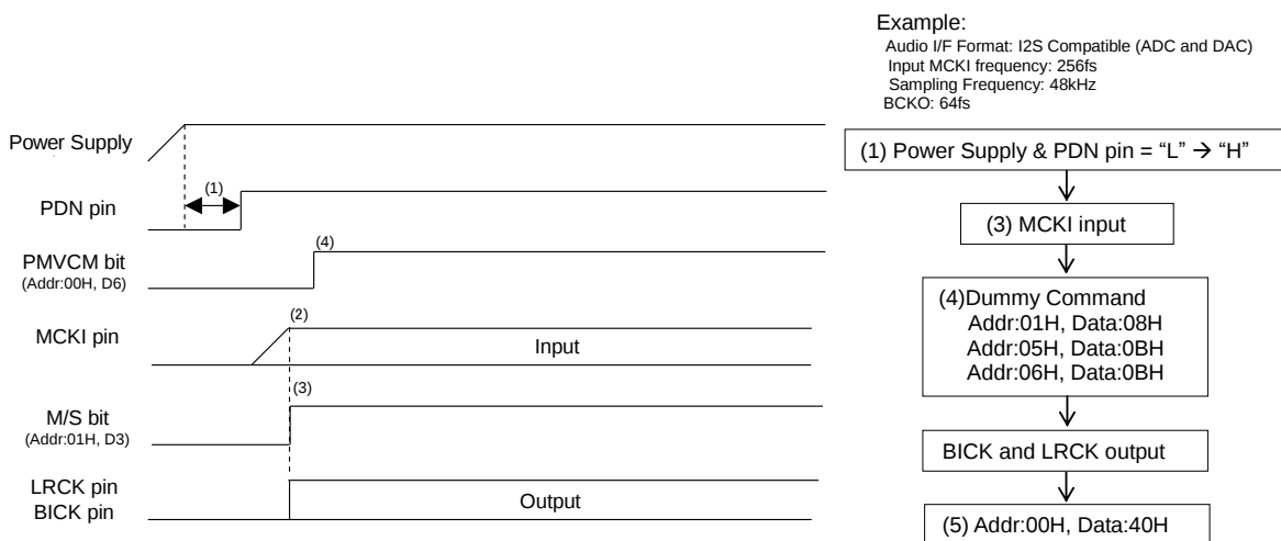
Figure 62. Clock Set Up Sequence (4)
