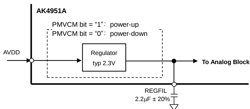
Figure 48 Regulator Block
