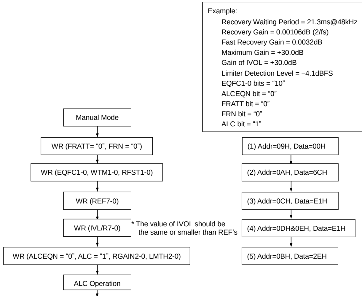
Figure 39. Registers Set-up Sequence at ALC Operation (Recording path)
