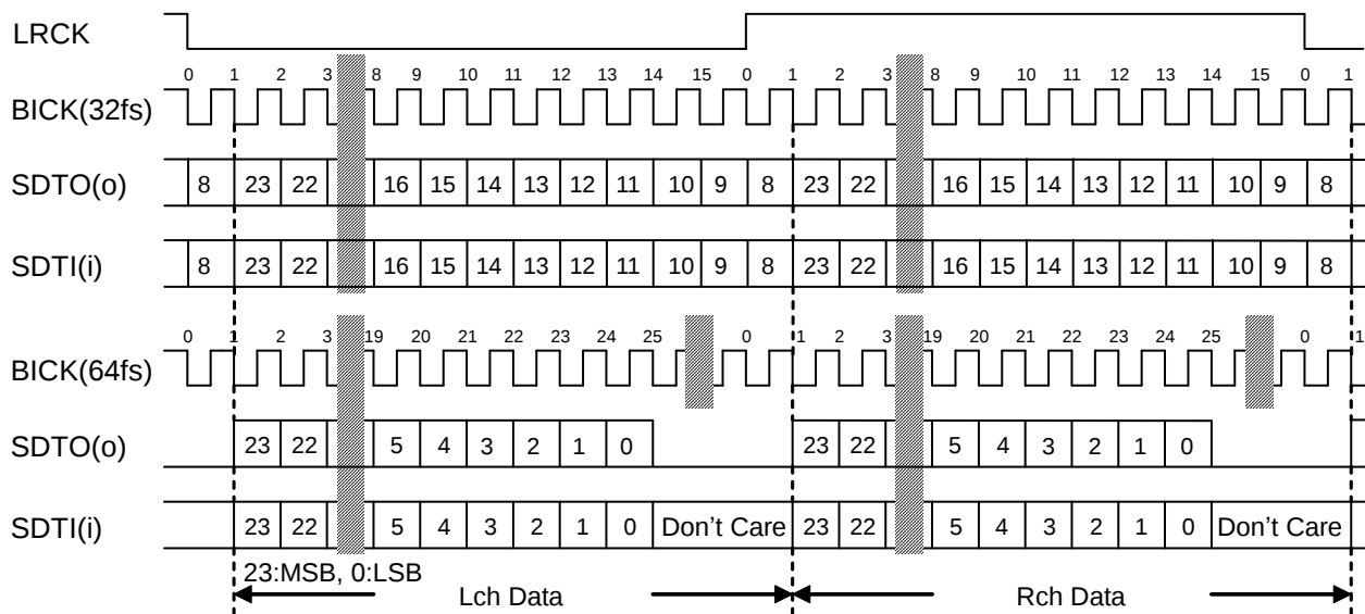
Figure 24. Mode 3 Timing
