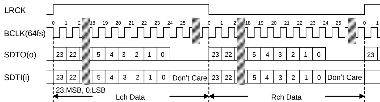
Figure 23. Mode 2 Timing
