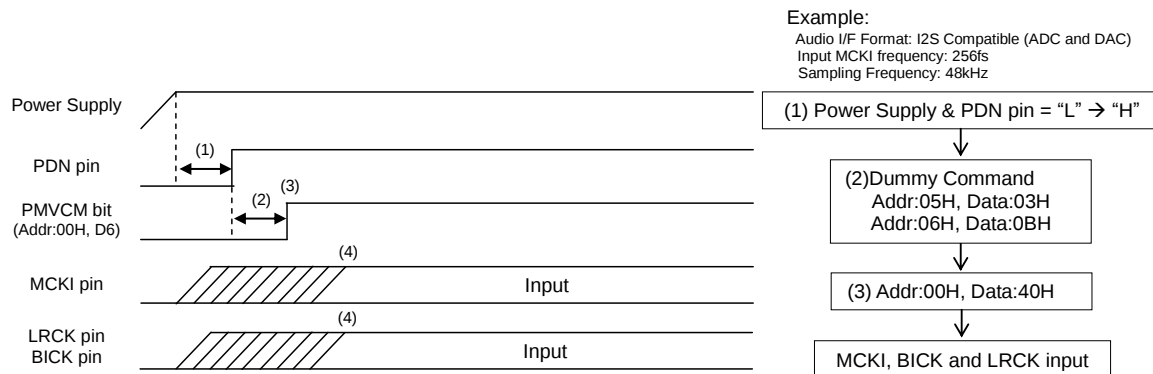
Figure 61. Clock Set Up Sequence (3)
