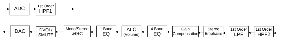
Figure 32. The Path in Recording Mode 2 &amp; Playback Mode 1
