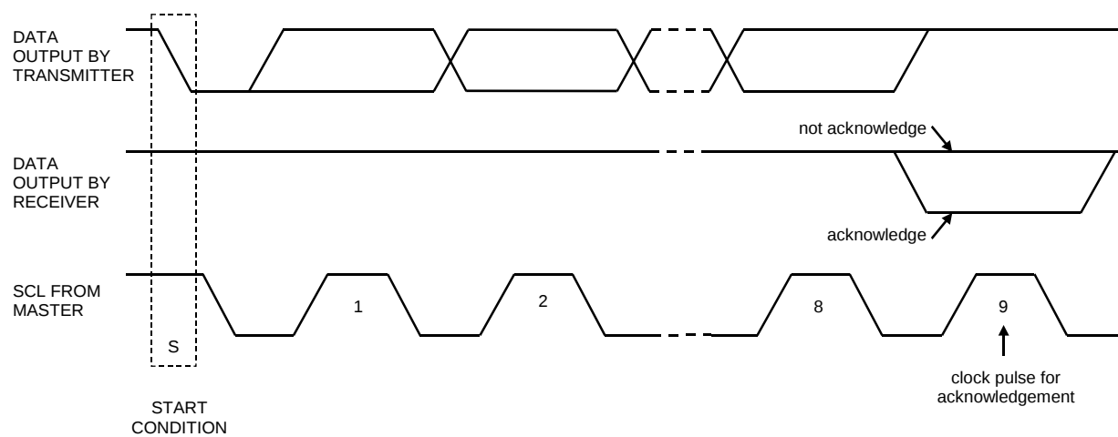
Figure 56. Acknowledge (I 2 C Bus)
