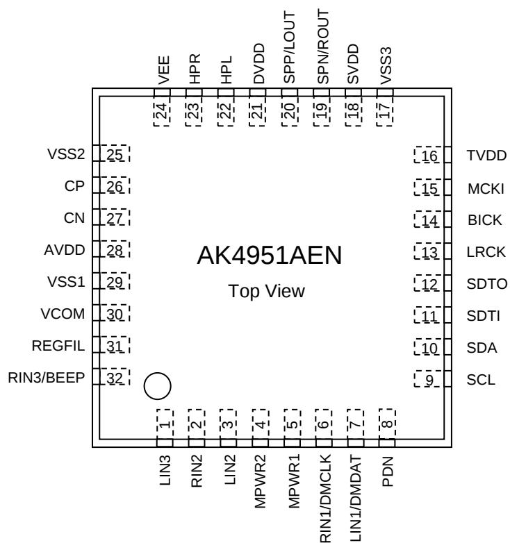
Figure 2. Pin Layout
