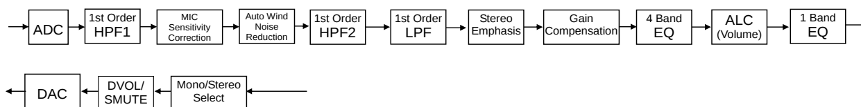
Figure 31. The Path in Recording Mode 1 &amp; Playback Mode 2 (default)
