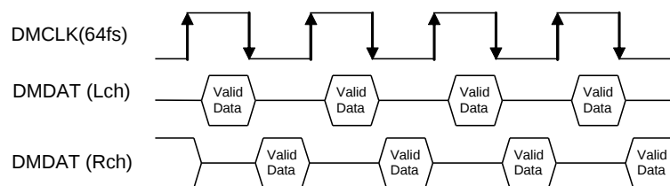
Figure 28. Data In/Output Timing with Digital Microphone (DCLKP bit = "1")
