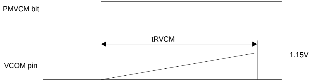
Figure 14. VCOM Rising Timing
