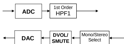
Figure 33. The Path in Recording Mode 2 &amp; Playback Mode 2
