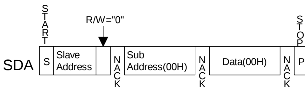
Figure 19. Dummy Command in I 2 C Bus Mode
