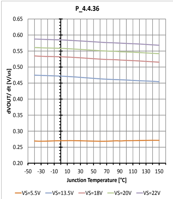
Slew rate OFF of low-side outputs
