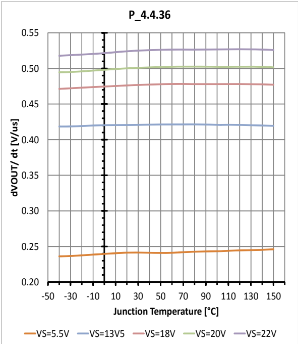
Slew rate OFF of high-side outputs
