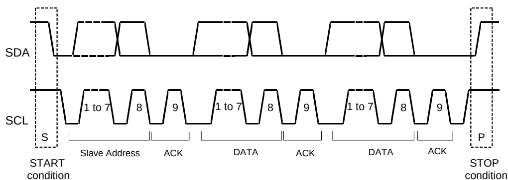
Figure 12. Acknowledge Timing
