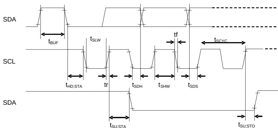
Figure 7. Interface Timing
