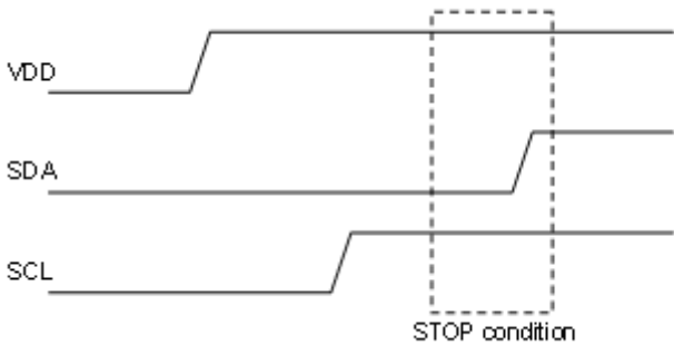
Figure 20. Stop Condition
