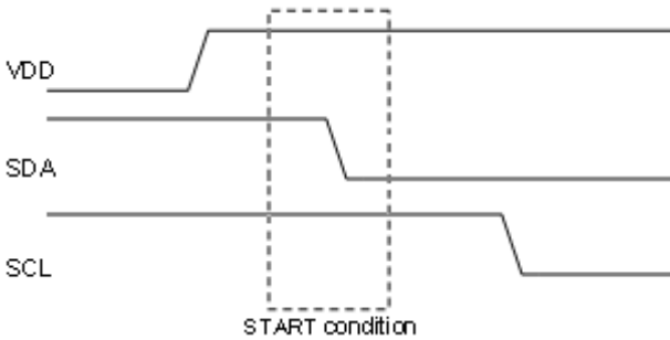
Figure 21. Start Condition
