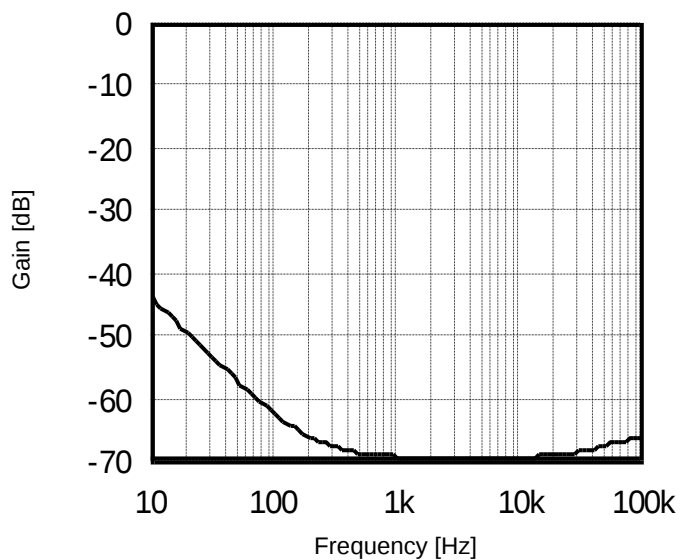
Figure 17. CMRR vs Frequency
