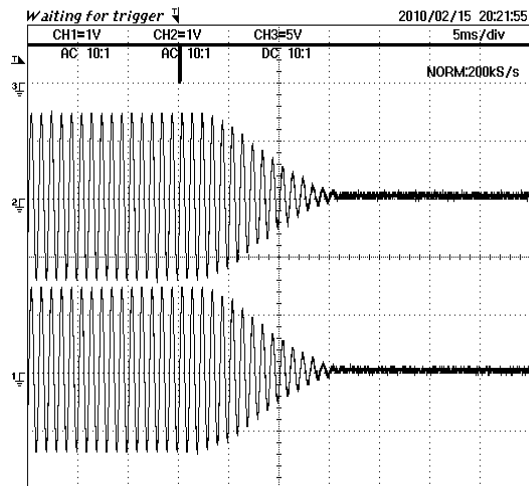
Figure 20. Advanced Switch 2
