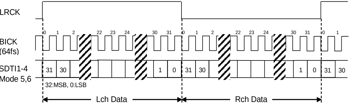
Figure 15. Mode 5/6 Timing
