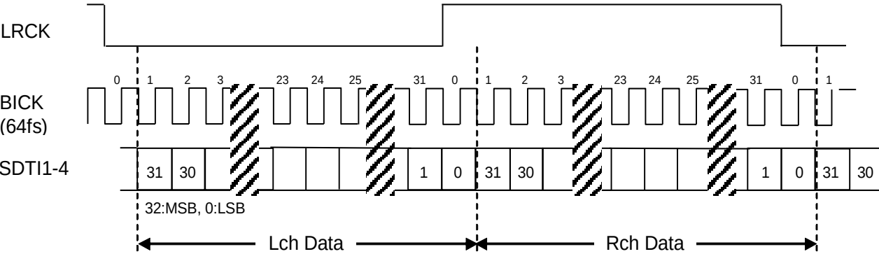
Figure 16. Mode 7 Timing
