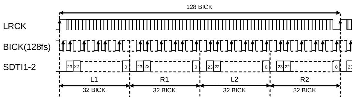
Figure 19. Mode 10 Timing
