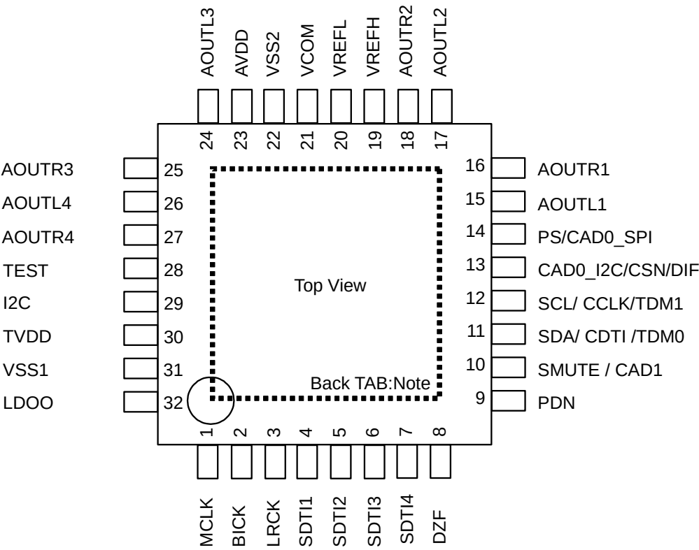
Figure 2. Pin Configurations
