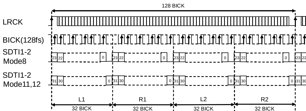
Figure 17. Mode 8/11/12 Timing
