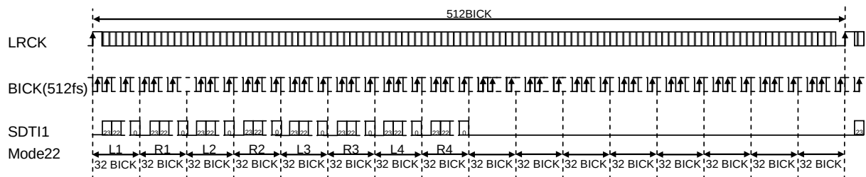
Figure 25. Mode 22 Timing
