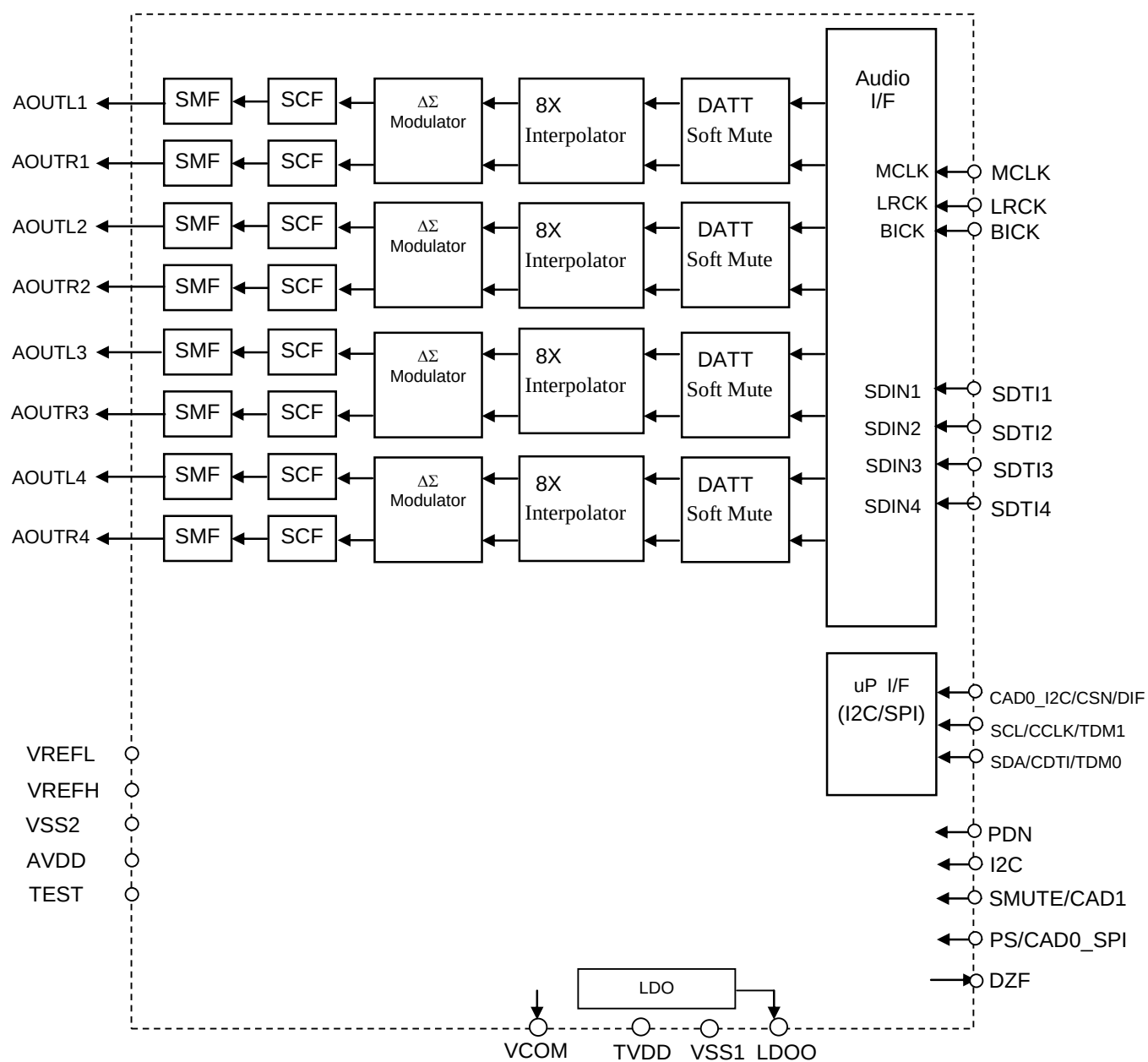
Figure 1. Block Diagram
