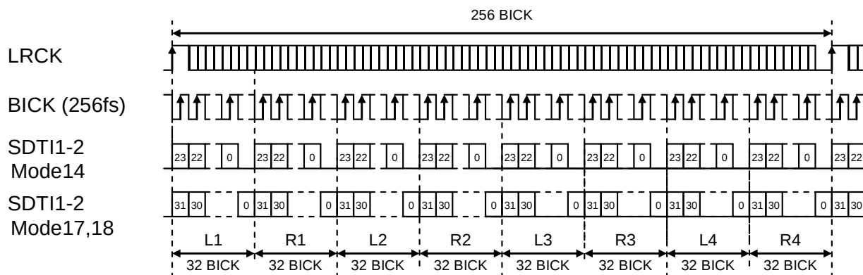
Figure 20. Mode 14/17/18 Timing
