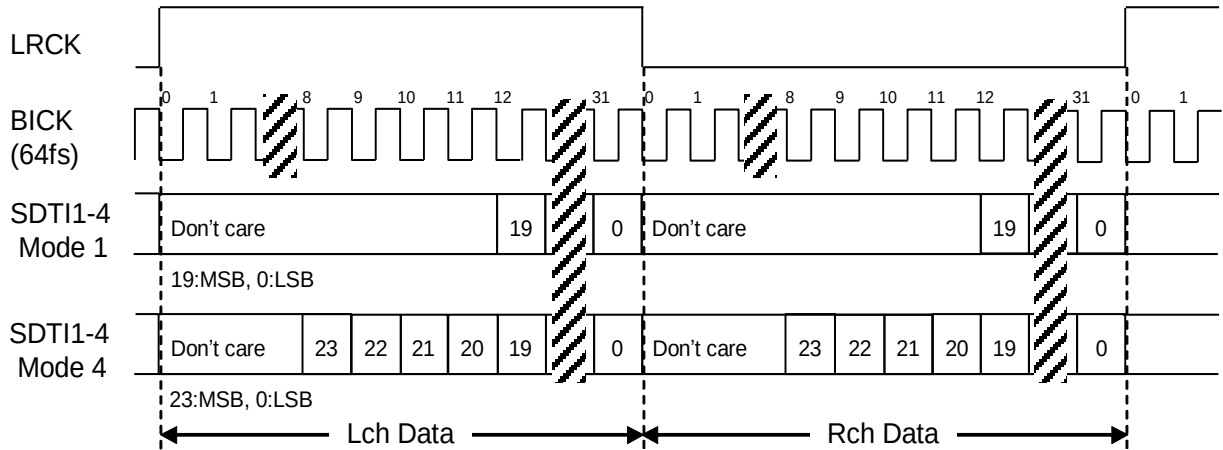
Figure 12. Mode 1/4 Timing
