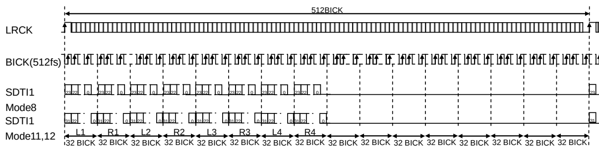
Figure 23. Mode 20/23/24 Timing
