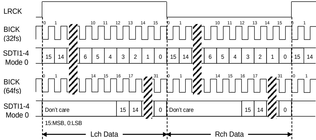
Figure 11. Mode 0 Timing
