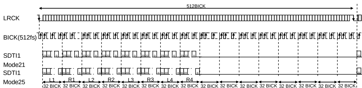
Figure 24. Mode 21/25 Timing
