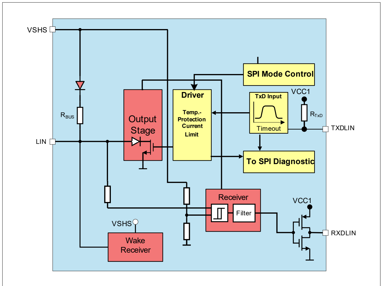
Figure 37 Block Diagram
