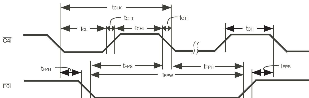
Figure 6. Clock Timing
