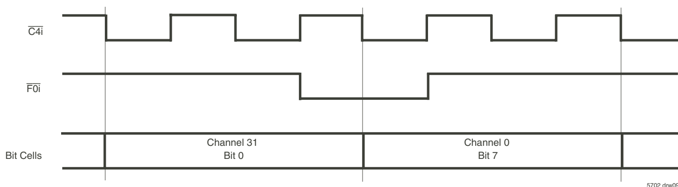
Figure 5. Frame Alignment
