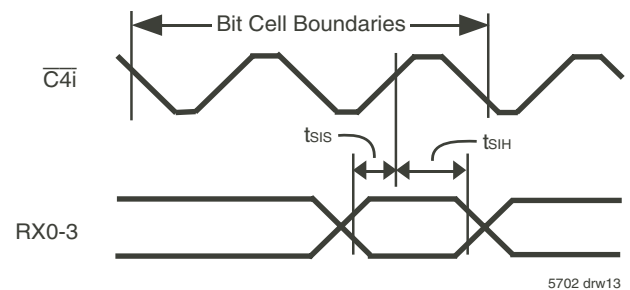
Figure 9. Serial Inputs
