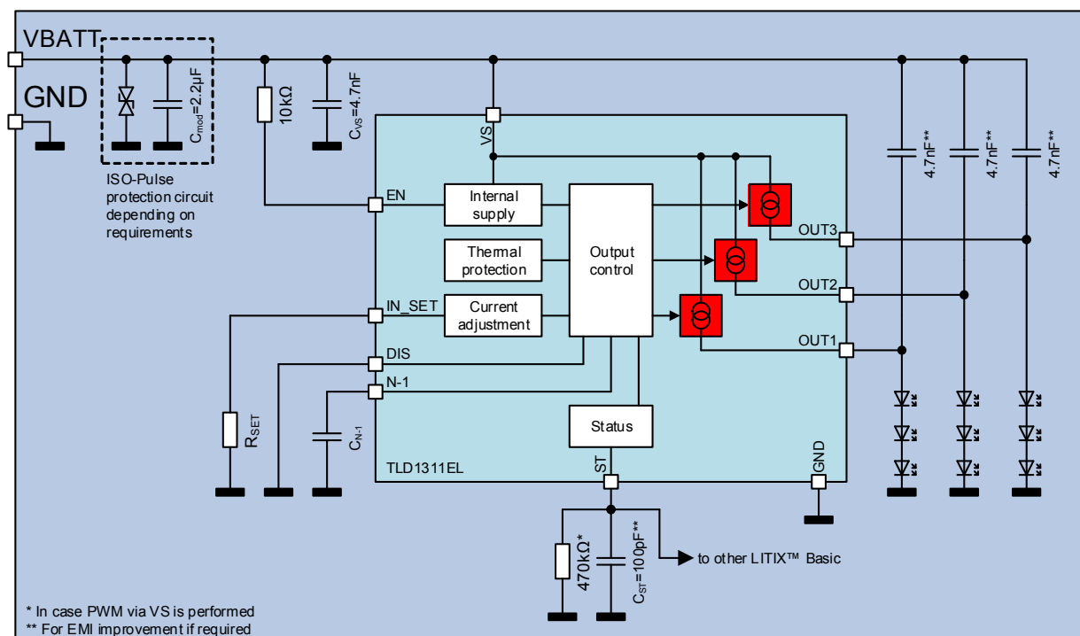
Application Diagram with TLD1311EL
