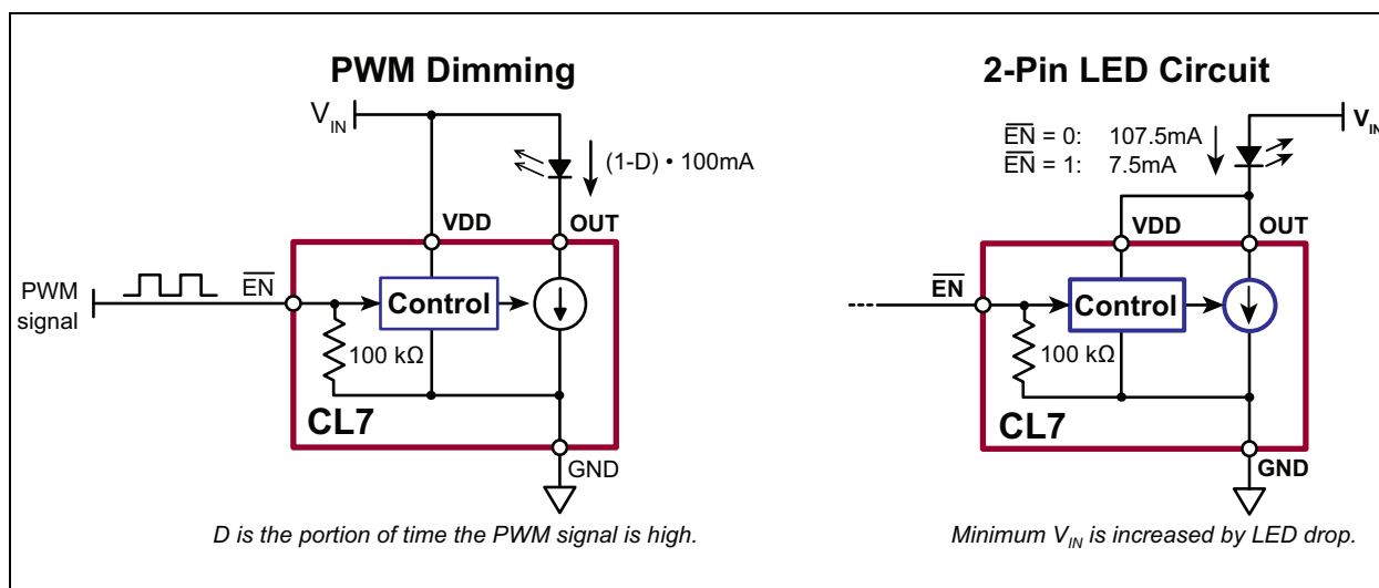
FIGURE 3-1: Application Circuits.
